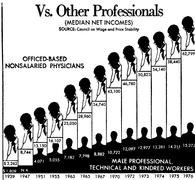
Figure 13. Changing scale in mid-axis to make exponential growth linear (© The Washington Post).
