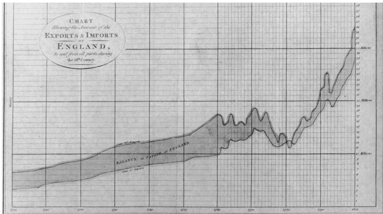
Figure 8. A plot on the same topic done well two centuries earlier (from Playfair 1786).
