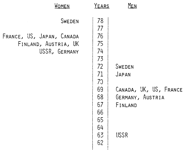
Figure 20. Ordering and spacing the data from Figure 19 as a stem-and-leaf diagram provides insights previously difficult to extract (from SI3).
