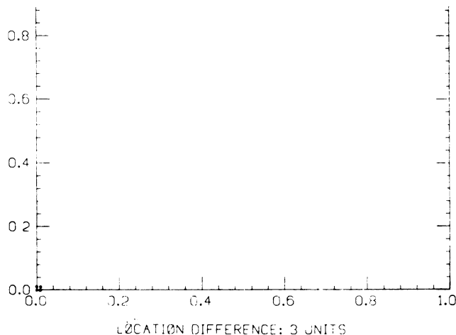
Figure 2. A low density graph (from Friedman and Rafsky 1981 [ddi = .5]).
