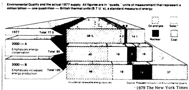
Figure 6. Ignoring the visual metaphor (© 1978, The New York Times).
