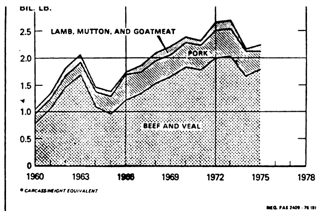
Figure 17. Jiggling the baseline makes comparisons more difficult (from Handbook of Agricultural Charts).
