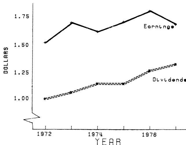
Figure 24. Data from Figure 23 redrawn simply (from Wainer 1980).
