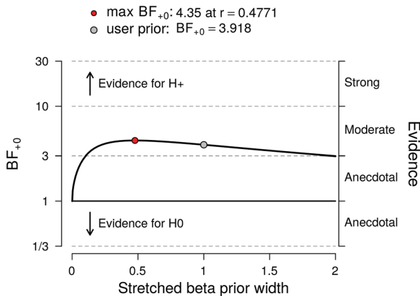
Figure 8. Sensitivity analysis for the Bayesian one-sided correlation test. The Bayes factor BF_{+0} is a function of the prior width parameter 1/a from the stretched \text{Beta}(a, a) distribution. Figure from JASP.
