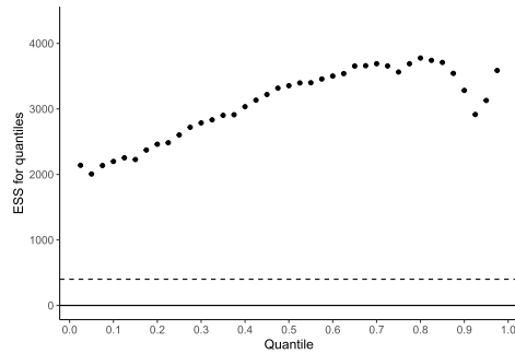
Figure 16: Efficiency of quantile estimates of \tau for the eight schools model with the non-centered parameterization. The dashed line shows the recommended threshold of 400.
